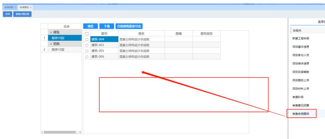
图：合格图纸
